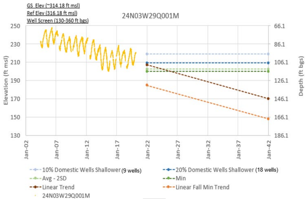
Figure 6A 3. Example Hydrograph Comparing Water Levels with Surrounding Approximate Domestic Well Depths
