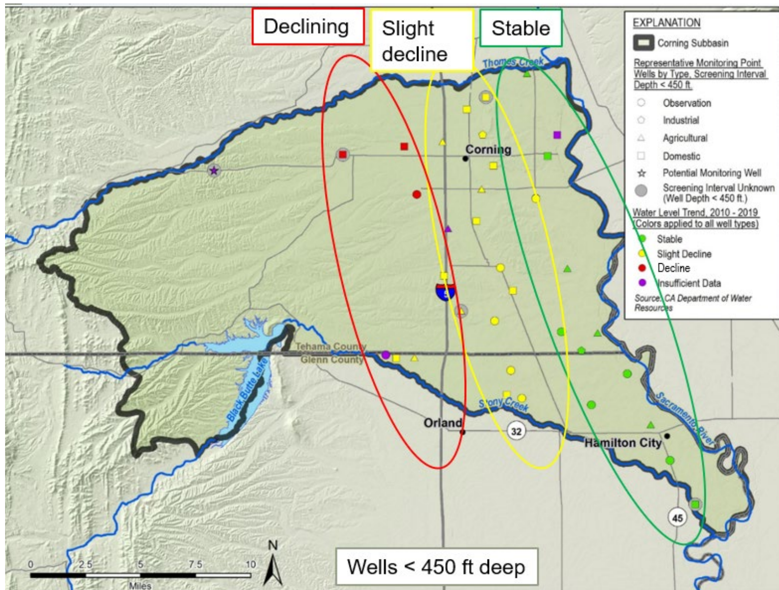
Figure 6-1. Qualitative Groundwater Level Trends at Shallow RMP Wells
