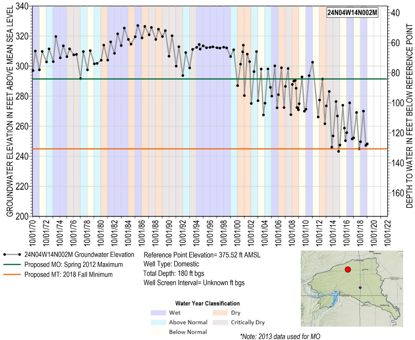
Figure 6A 4. Groundwater Level Hydrograph with Preliminary Potential Measurable Objective and Minimum Threshold
