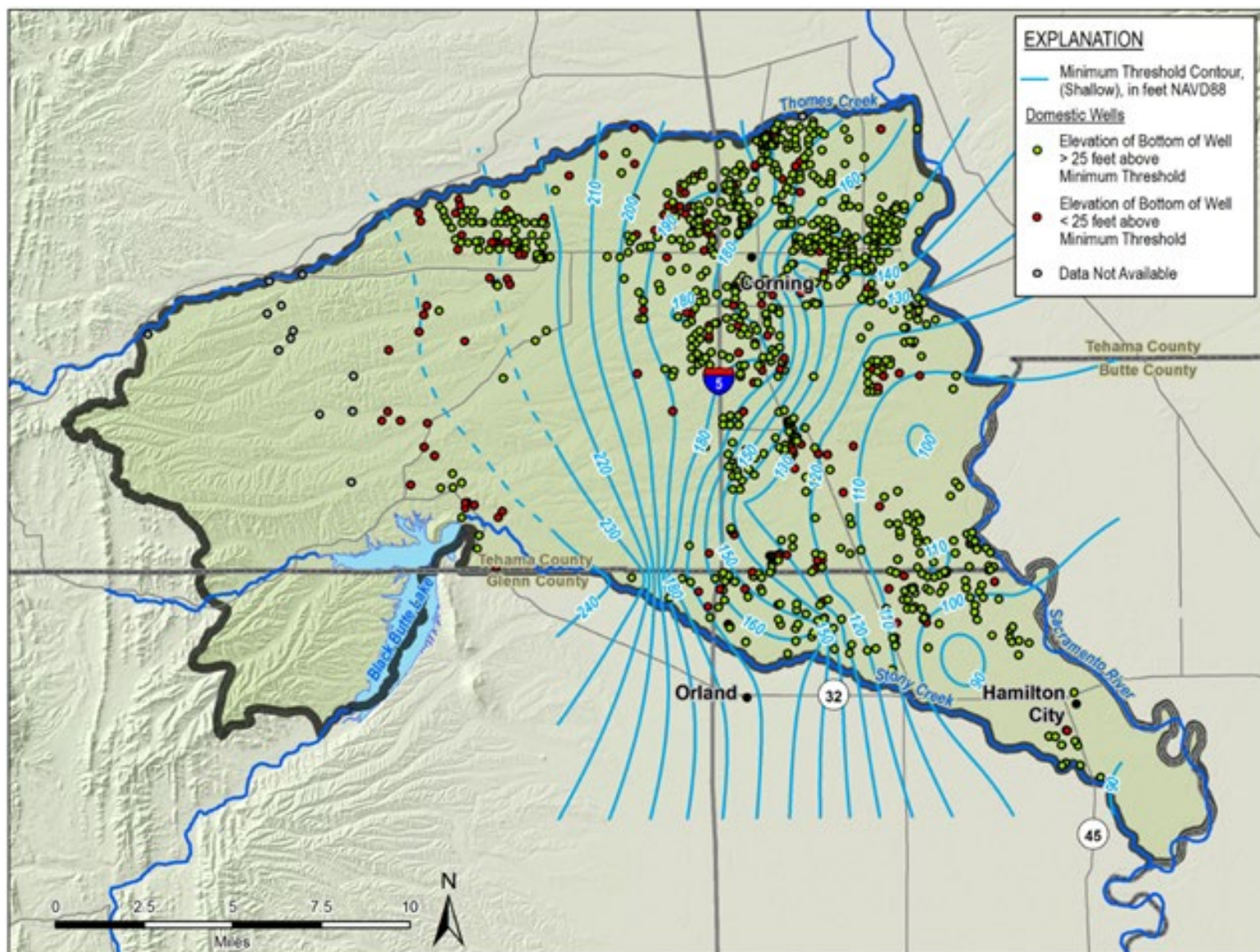
Figure 6-6. Domestic Wells at Risk of being Impacted if Water Levels Reach Minimum Thresholds
